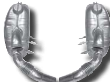
96.330S (1620602210) (OE 996.111.210.00) Rear sport exhaust set, OE style Polished stainless steel 304/4301 With TÜV/EEC approval
