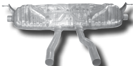
95.302S (1620611100) Sport exhaust without tail pipes Stainless steel 304/4301
