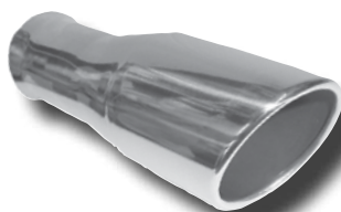
92.241S (1620701100) Tail pipe, Ø102 mm, flared angle end, clamp on type Polished stainless steel 304/4301
